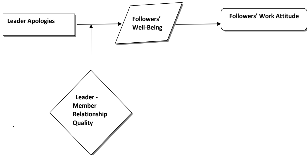
Figure 1. Theoretical framework.
